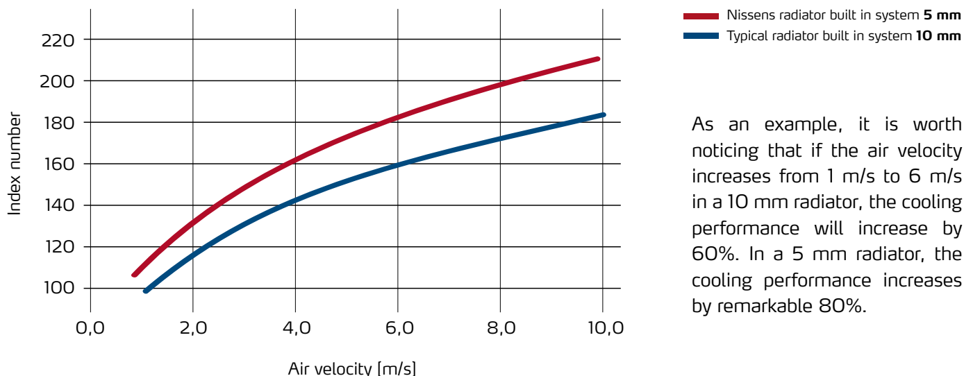
Comparison between radiators in systems 5 mm and 10 mm
